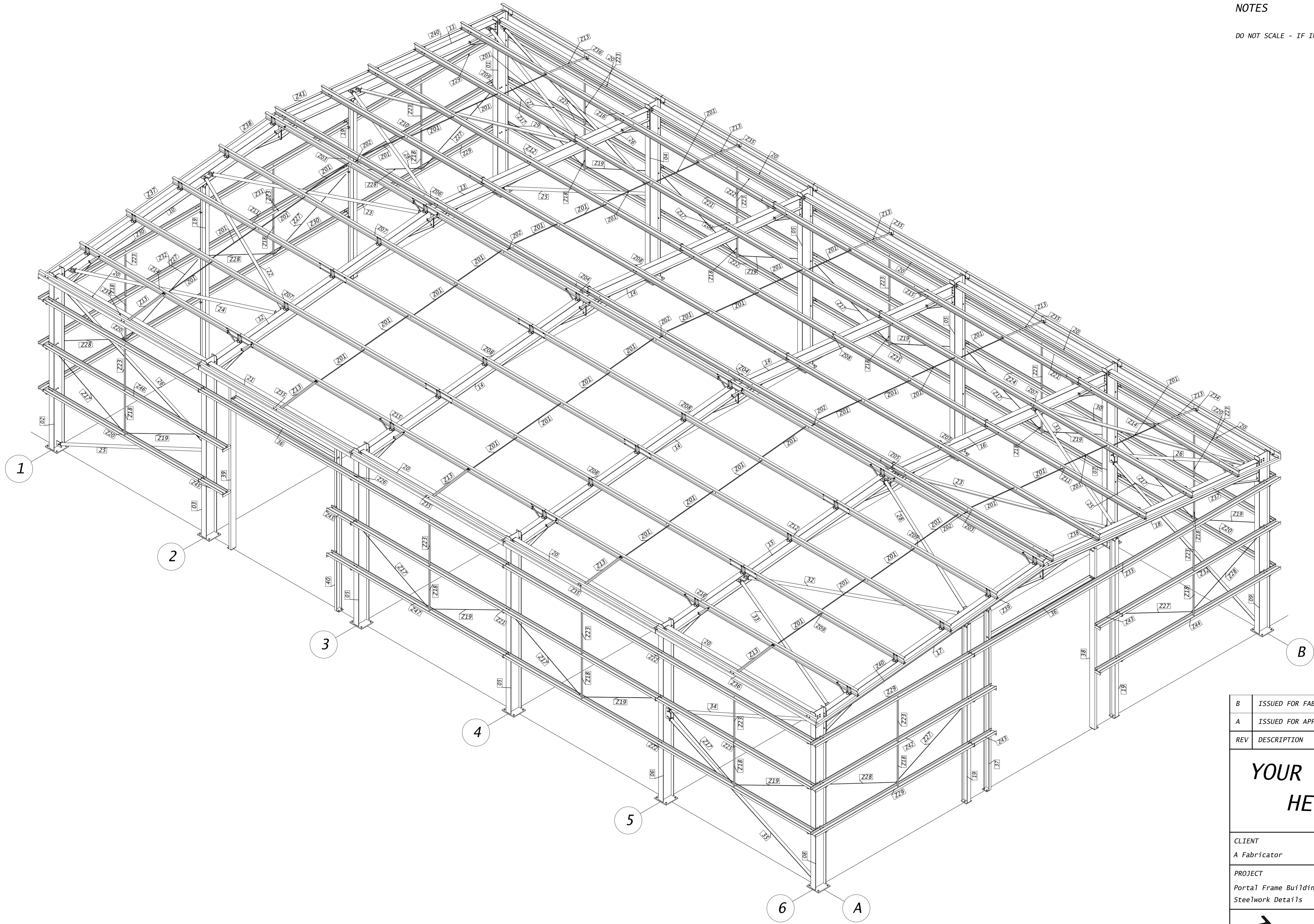
3-D VIEW
